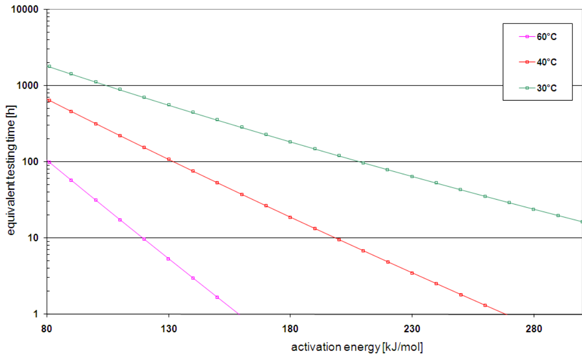
Figure 1 Equivalent testing times for the absorber tested for different testing temperatures. As initial testing temperature 40°C has been selected. Thus, the maximum testing time was determined to be 600h, corresponding to a minimum activation energy of 80kJ/mol.
